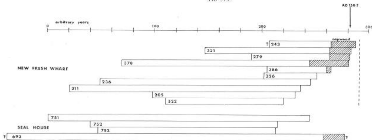
Fig. 1: Block diagram showing the arbitrary years spanned by each timber of the Roman waterfronts at New Fresh Wharf and Seal House. Hatching indicates the presence of sapwood which allows an estimation of the felling date (vertical dotted line) and construction date. The scale in arbitrary years may correspond approximately to 130 BC to AD 150; dating is being checked by four C14 dates from positions shown by brackets at the base.
